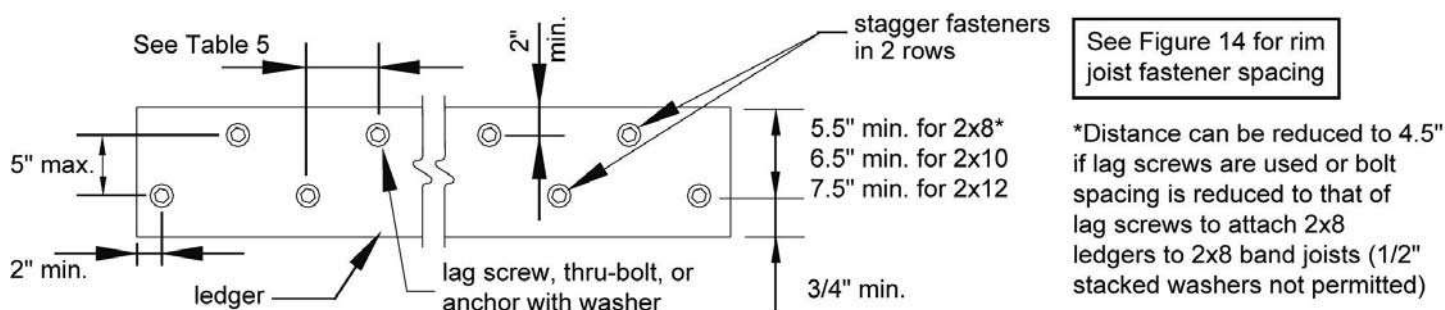
Figure 19: Ledger Board Fastener Spacing and Clearances
