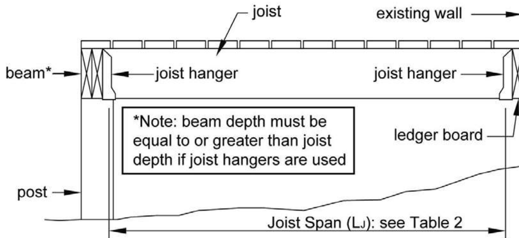
Figure 2. Joist Span – Free Standing Deck
